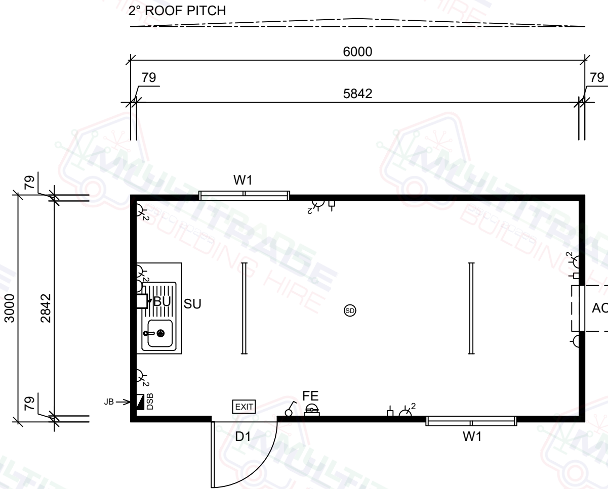
6.0x3.0m Crib Room - Floor Plan
